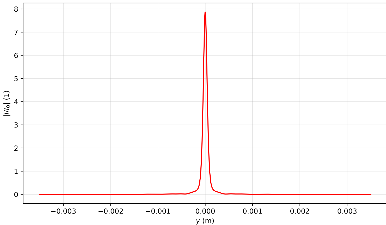
Intensity profile I(x=0, y, z=3.662)/I_0 , P_{in}=4.0P_{cr} , artificial time
